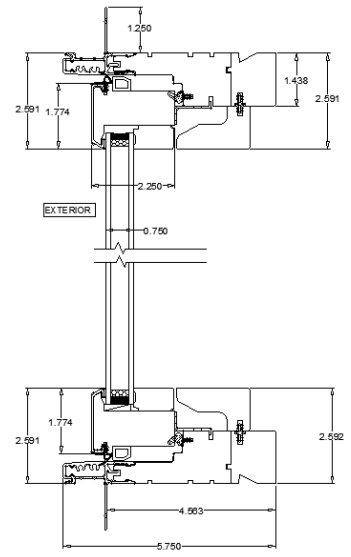
VERTICAL SECTION – TRANSOM Narrow Sash
